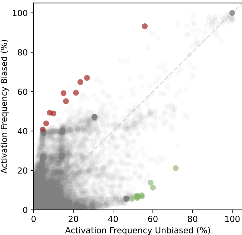
Activation Frequencies of SAE Latents: Bbq_race
